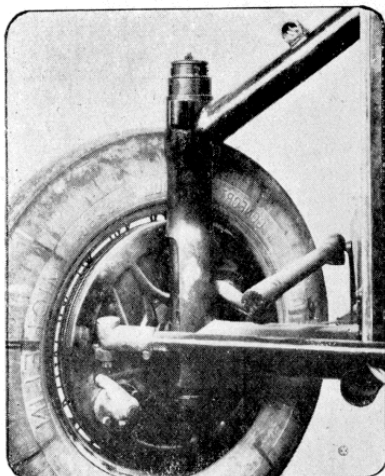
Fig. 4. — Suspension avant.
